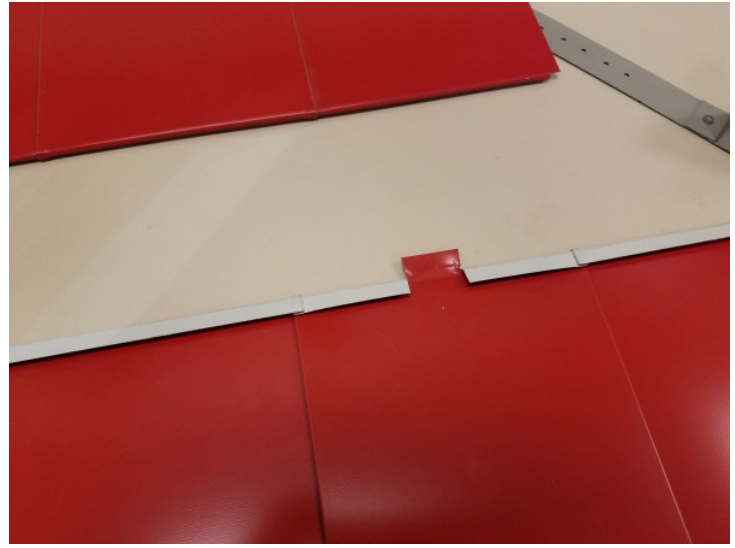
Bend the seam open and flatten it to the roof
