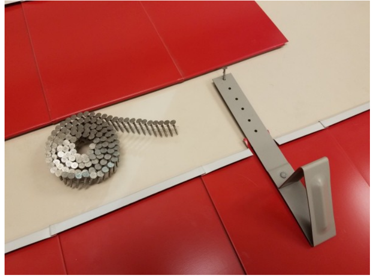
Use ring shank nails or screws to fasten the snow hook with at least 4 fasteners
